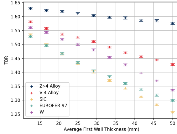
Figure 9: TBR degradation as a function of first wall thickness for various candidate materials, including EUROFER97 [53], Zr-4 as defined in Section 4.3.2 and the rest defined in [52]. Zirconium-based alloys demonstrate the highest TBR profile.
