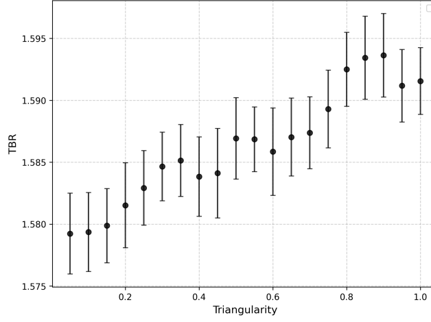
Figure 8: Sensitivity of TBR to reactor triangularity ( \delta ). Noting the y-scale, the gradient of 0.015 \pm 0.001 indicates that triangularity has a negligible impact on global neutronics, consistent with the use of a uniform ring source model.
