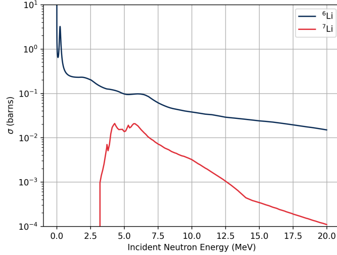
Figure 2: A graph of the tritium production cross-sections of {}^6\text{Li} and {}^7\text{Li} . Cross-section data was acquired from ENDF B/VIII.1 (Brown et al., 2018).
