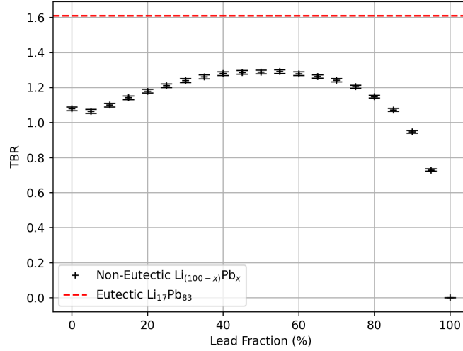
Figure 5: A plot of the TBR for a series of non-eutectic lithium-lead mixtures in comparison with eutectic \text{Li}_{17}\text{Pb}_{83} .
