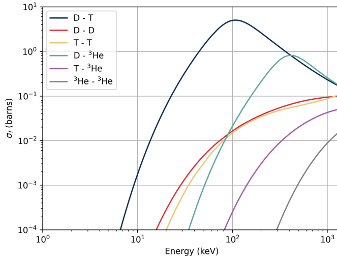
Figure 1: A graph showing the fusion cross-sections ( \sigma_f ) of several fusion reactions for a range of energies. The cross-section data for this graph was collated by the Brookhaven National Laboratory for the Evaluated Nuclea Data File (ENDF B/VIII.1) (Brown et al., 2018).
