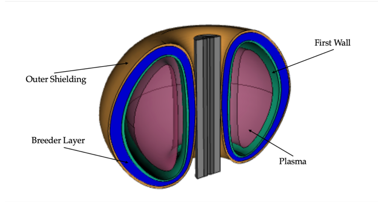
Figure 4: A visual representation of the simple Tokamak design used in our simulations. This design was imported from the Paramak library of fusion reactor structures created by Shimwell et al. (2021). Key structures are labelled in the figure.
