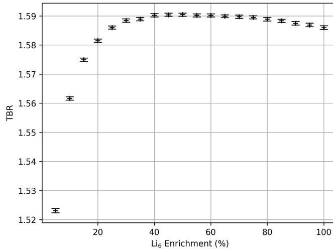
Figure 6: This graph depicts the change in TBR for a range of ^6\text{Li} enrichment values. The enrichment is expressed in terms of molar fraction.
