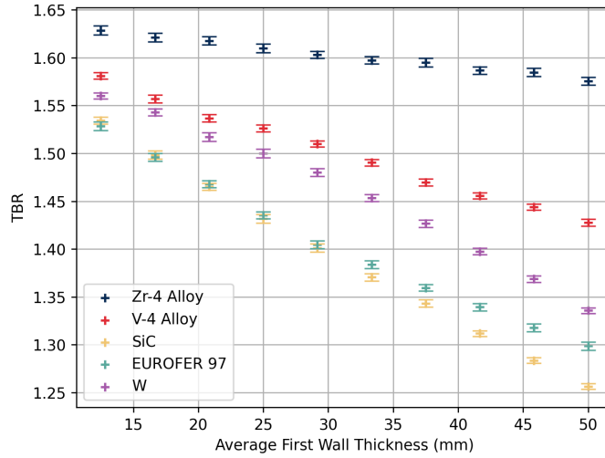
Figure 8: A graph showing how TBR changes with the thicknesses of several common first wall materials.
