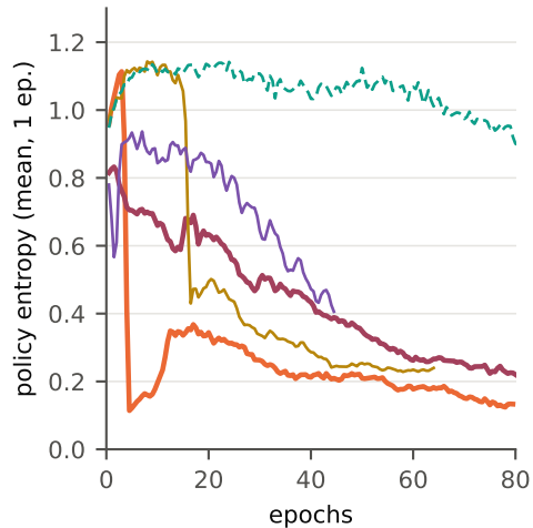
(c) entropy
