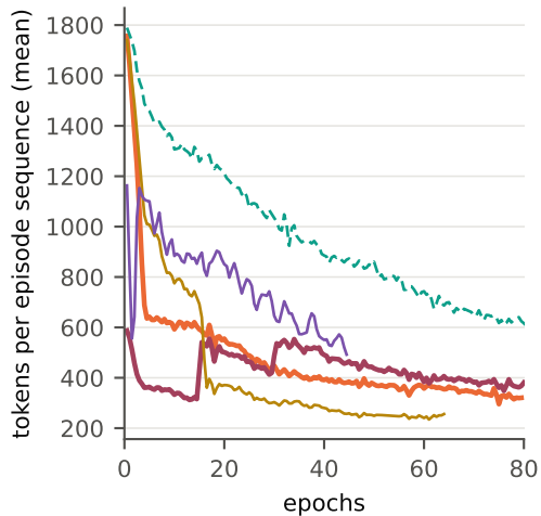
(b) episode length in tokens
