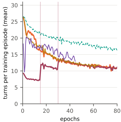
(a) episode length in turns
