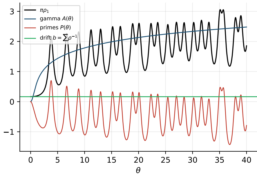
Thorin density from the sine squared lemma
