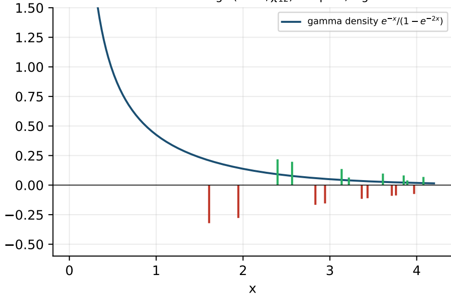
Canonical measure of \log \Lambda(1+s, \chi_{12}) : no pole, signed atoms
