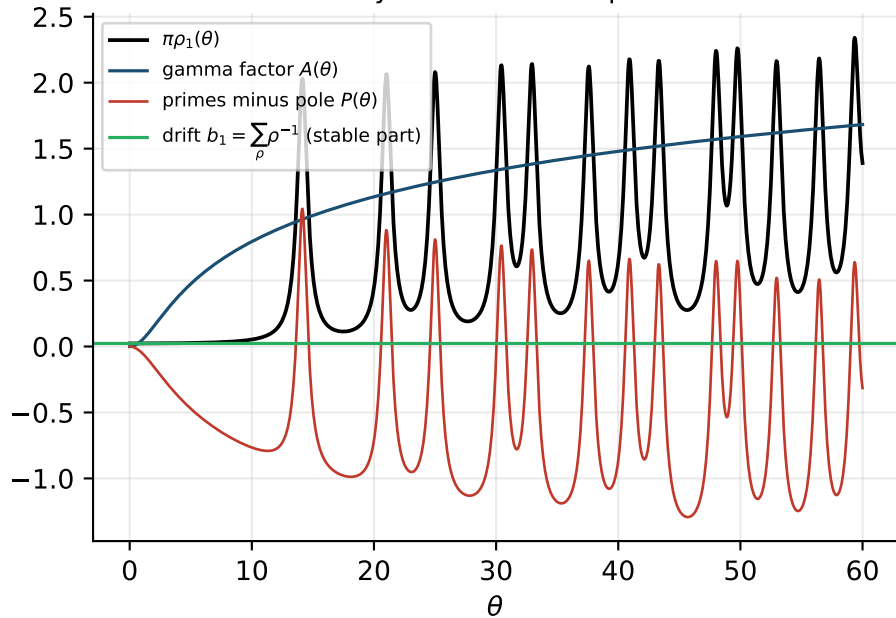
Thorin density from the sine squared lemma
