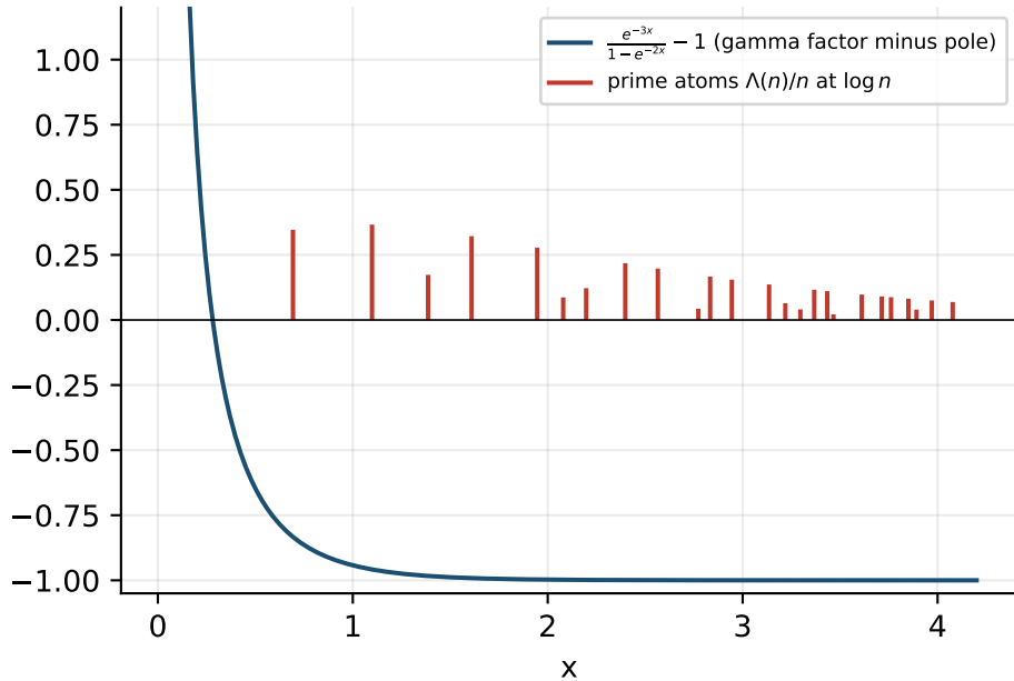
Signed canonical measure x\Pi_1(dx) of \log \xi(1+s)
