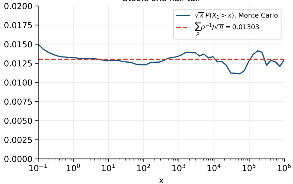
Stable one half tail
