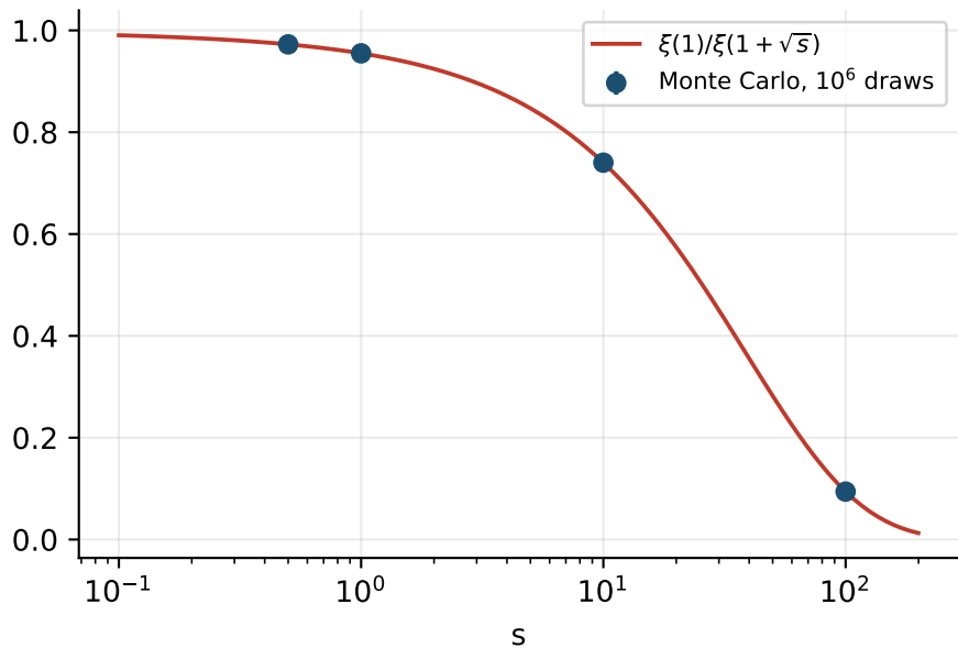
Laplace transform of \tilde{T} + H_{\tilde{T}/\sqrt{2}}
