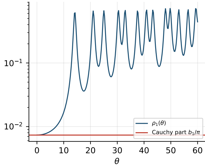
Thorin density of Y_1 and its Cauchy floor
