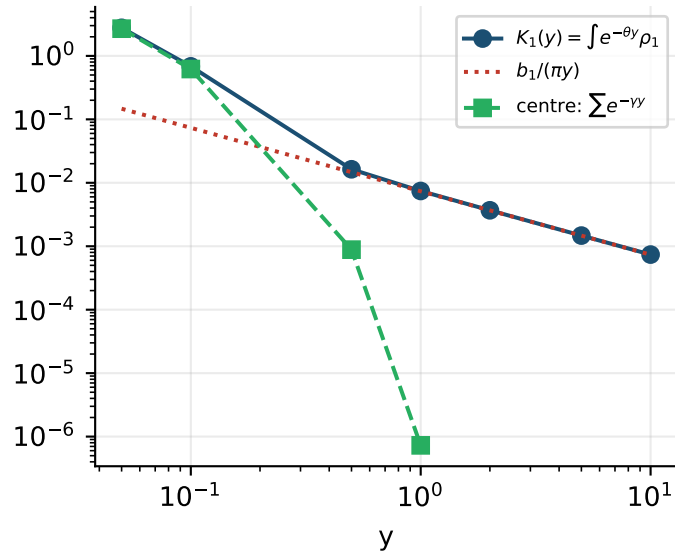
Lévy kernels: \nu_\alpha(y) = K_\alpha(|y|)/|y|
