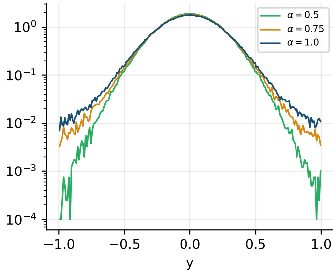
Density of Y_\alpha = \sqrt{2X_\alpha} Z
