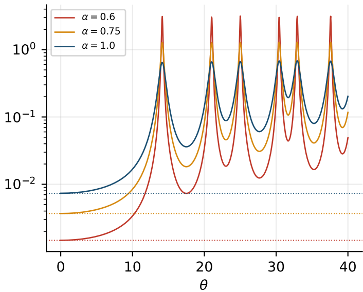
\rho_\alpha in the strip, Cauchy floors b_\alpha/\pi
