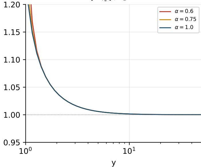
\pi y^2 f_{Y_\alpha}(y)/b_\alpha \rightarrow 1
