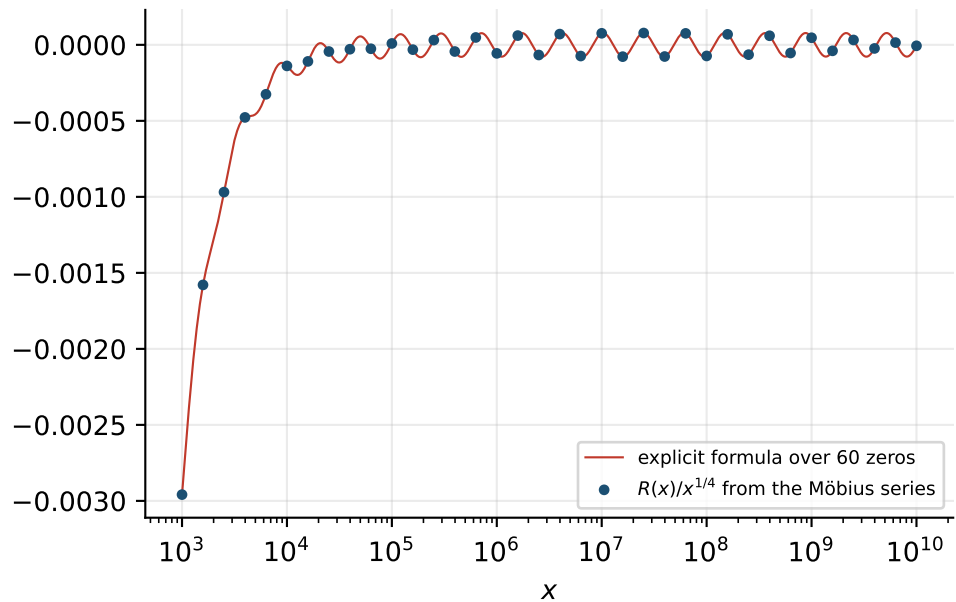
Riesz's criterion: R(x) = O(x^{1/4 + \delta})
