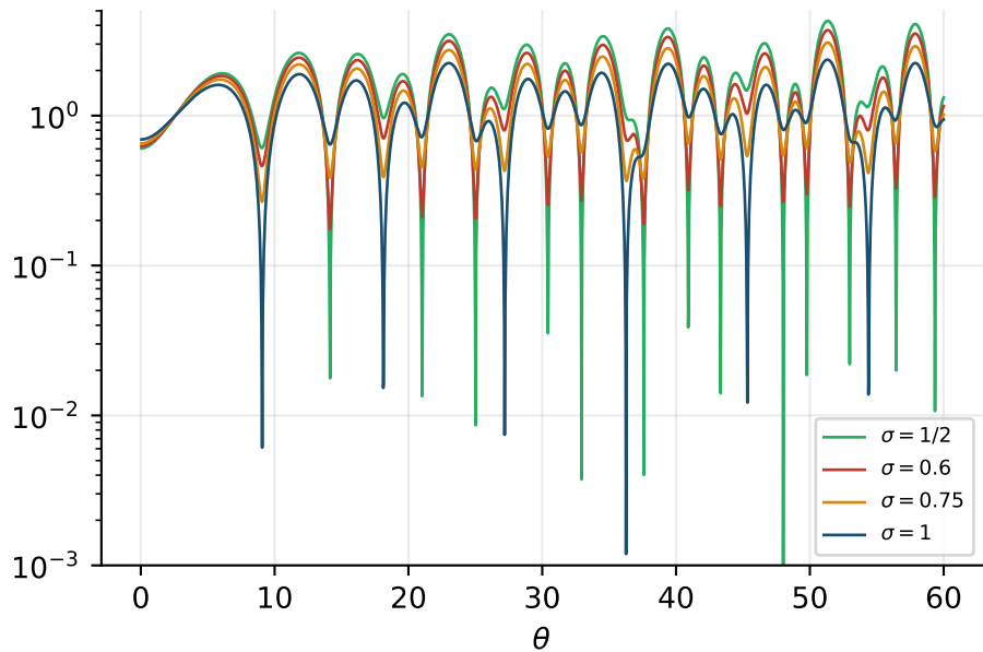
Salem kernel: |\eta(\sigma + i\theta)| on the lines \text{Re } s = \sigma
