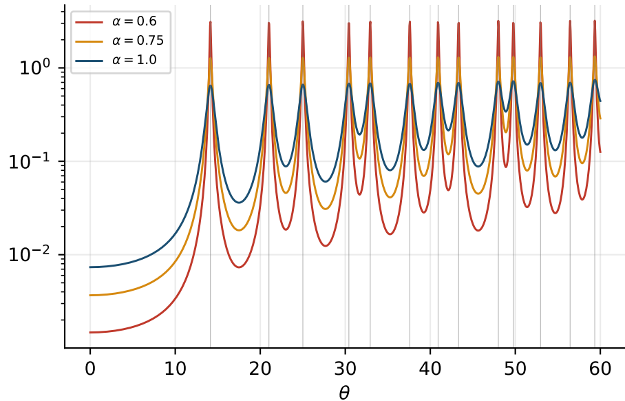
Thorin densities \rho_\alpha of \xi(\alpha)/\xi(\alpha + \sqrt{s})
