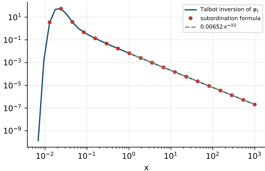
Density of X_1
