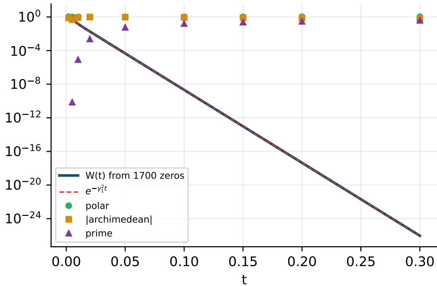
Heat trace and its arithmetic pieces
