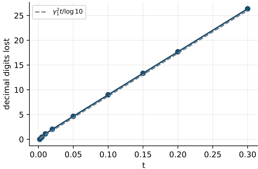
Cancellation in the explicit formula
