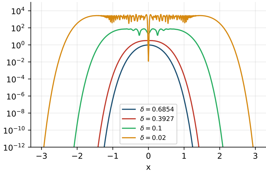
|\Phi(x + i(\pi/4 - \delta))| inside the strip
