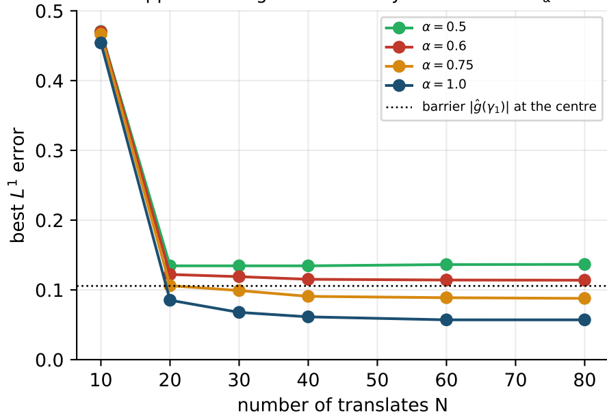
Approximating a Gaussian by translates of \Phi_\alpha
