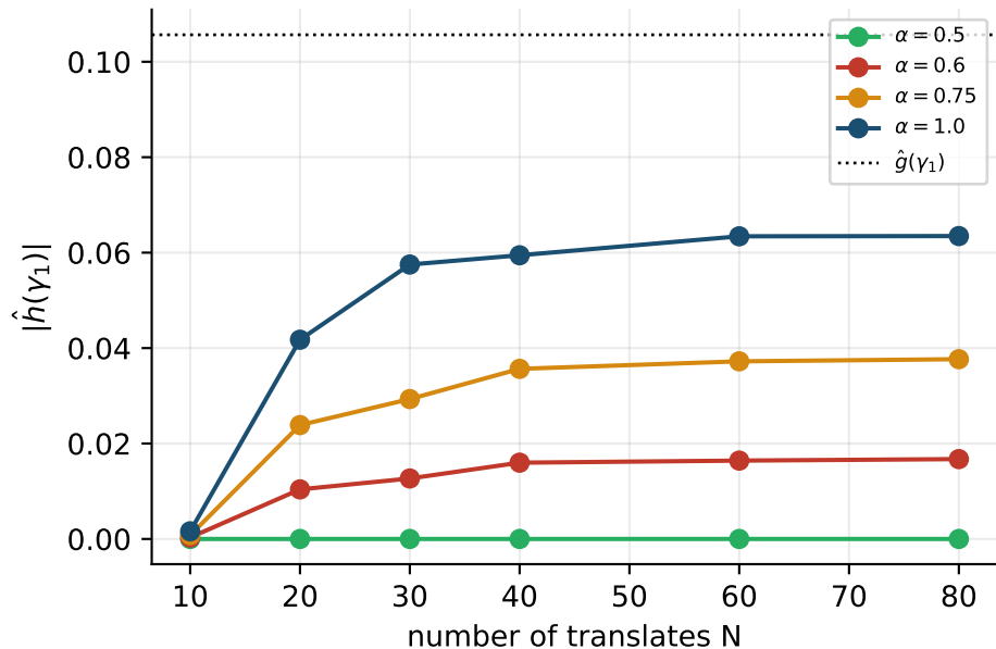
The approximant at the first ordinate
