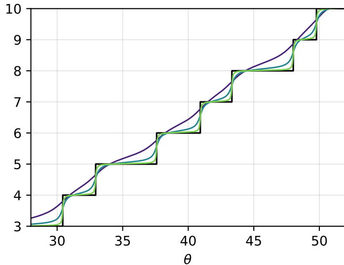
Cumulative Thorin mass against the counting measure of the squared ordinates
