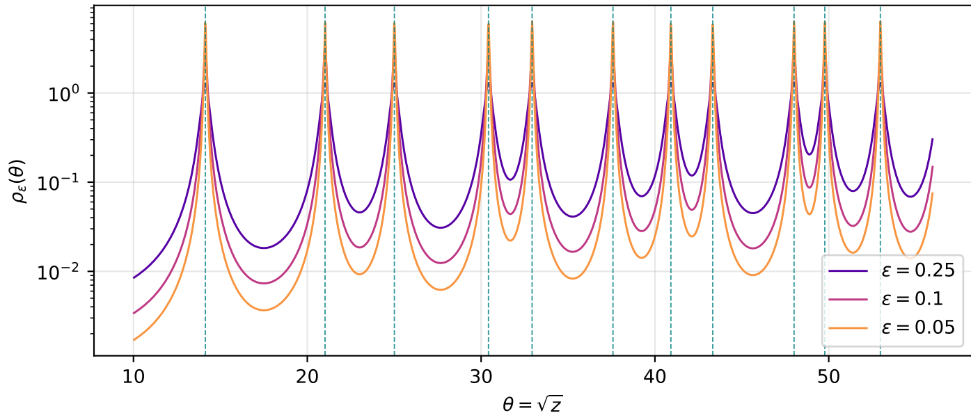
Pólya computed Thorin density at basepoint 1/2+\varepsilon (dashed: zero ordinates)
