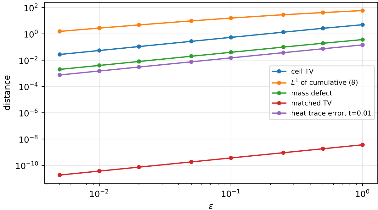
Distances to the RH measure on z \leq 200^2
