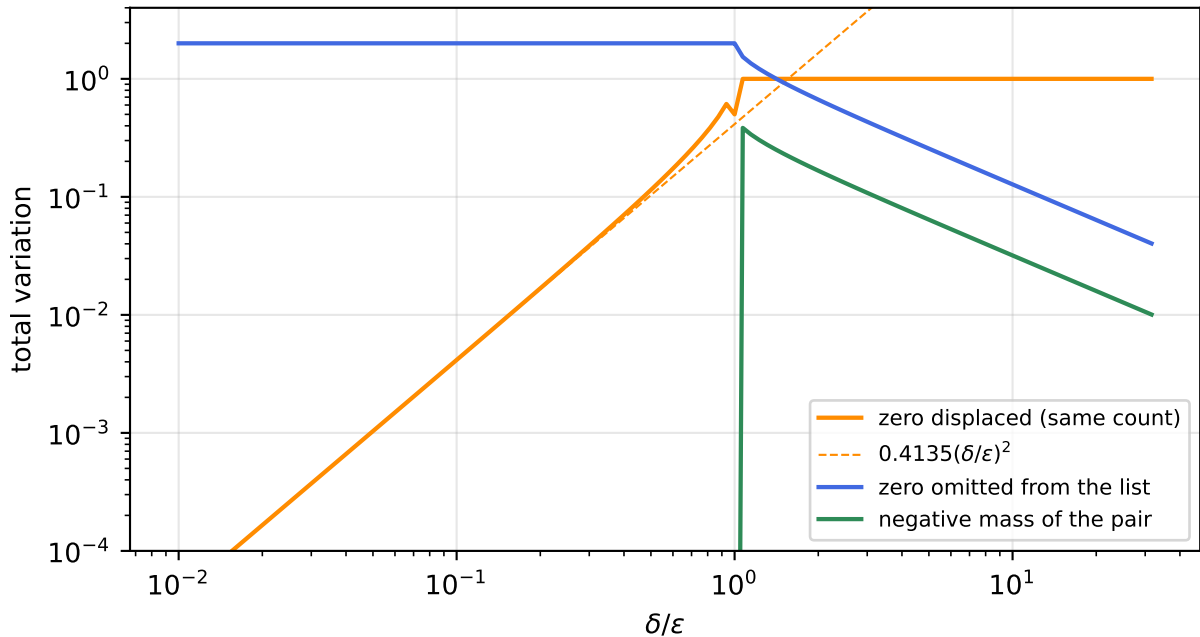
Signature of one off line pair at resolution \varepsilon
