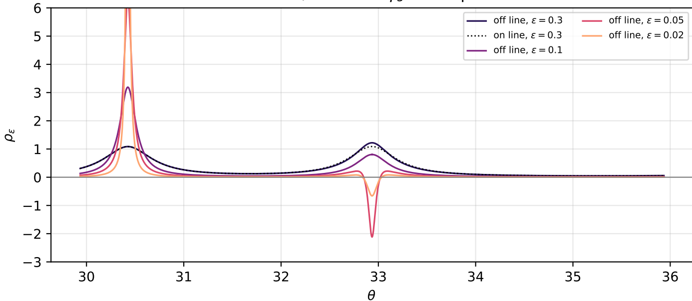
Fifth zero moved to 1/2 \pm 0.1 + i\gamma_5 : the dip vanishes as \varepsilon \rightarrow 0
