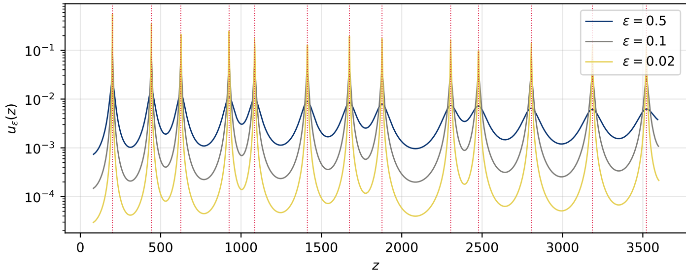
Thorin density in the clock variable z (dotted: \gamma^2 )
