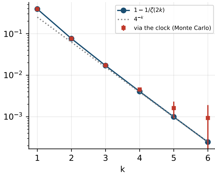
Riesz coefficients from the clock
