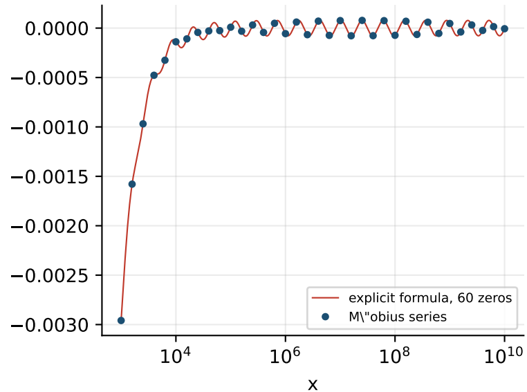
R(x)/x^{1/4}
