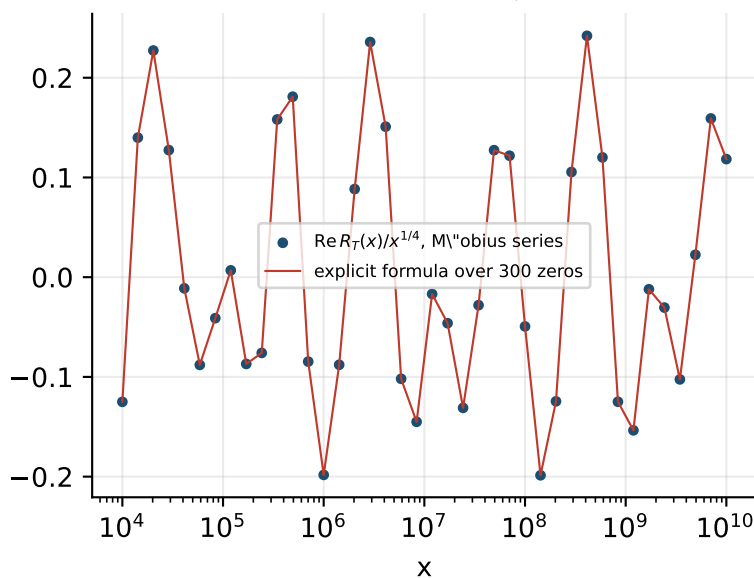
Twisted Riesz function, T = 50
