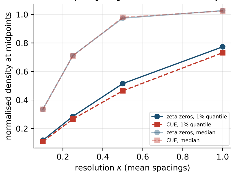
Positivity margins against random matrix theory
