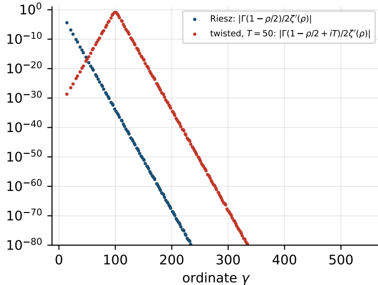
Which zeros a Riesz filter sees
