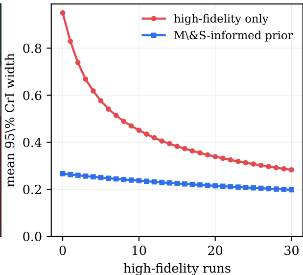
(b) A cheap prior sharpens costly tests
