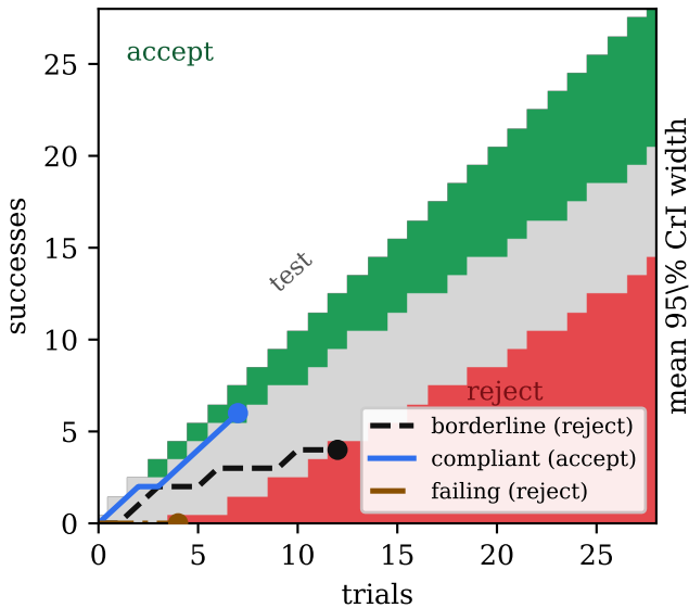
(a) Decision chart and evidence walks
