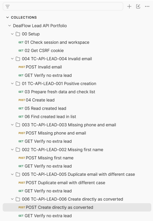
Figure 7. Collection structure captured during execution. Case numbers map to TC-API-LEAD-001 through TC-API-LEAD-006.
