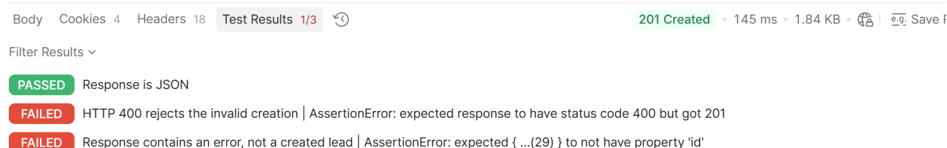
Figure 3. Two failed checks: expected HTTP 400, and expected an error without a created ID. JSON response validation passes.
