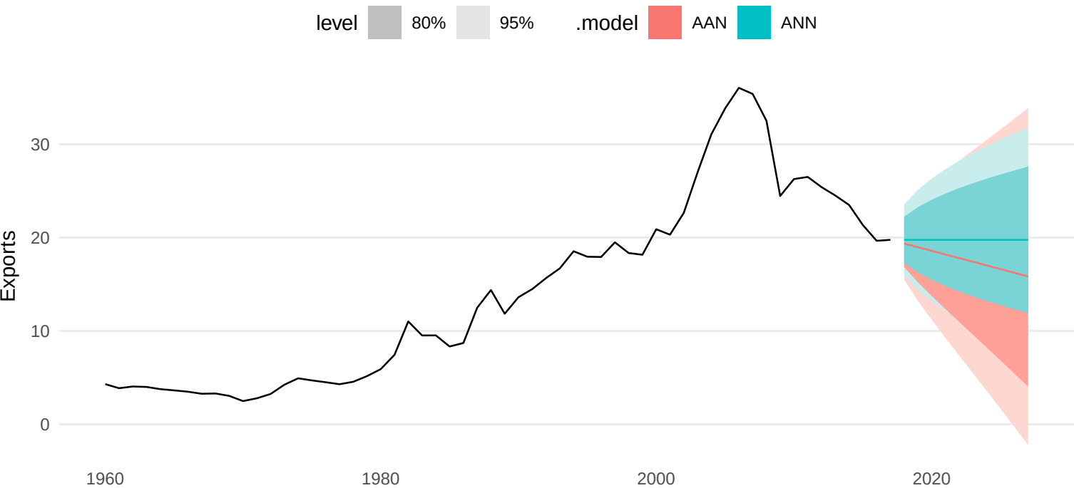
Exercise 5(d): ETS(A,N,N) versus ETS(A,A,N)
