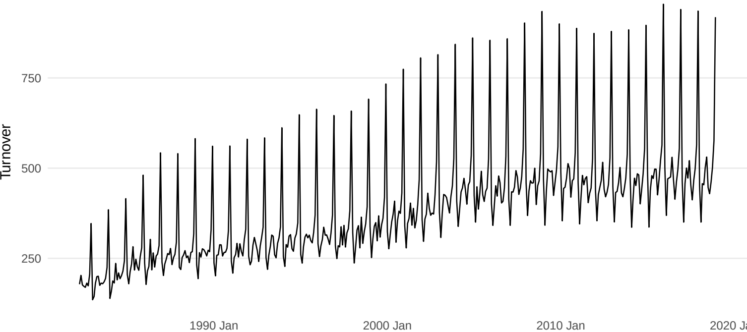
Chosen retail series: NSW department stores
