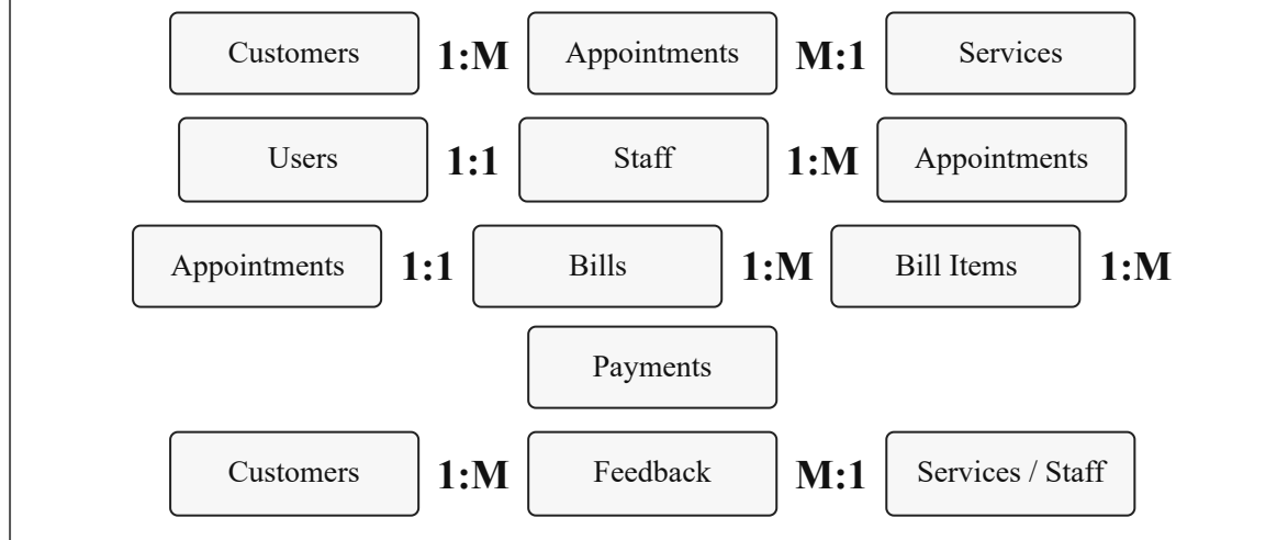
Figure 4.5: Entity Relationship Model
