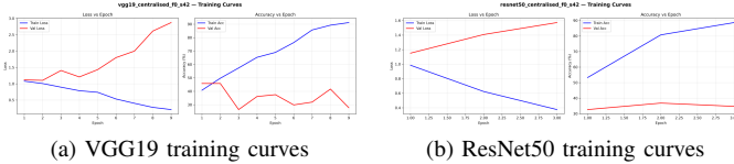
Fig. 3. Training loss and validation accuracy curves for centralised VGG19 and ResNet50 (subject-level fold 0, seed 42). Validation accuracy plateaus early and near chance level, consistent with the small number of distinct training subjects.
