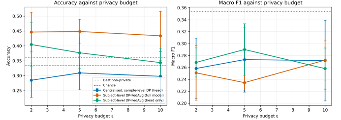
Fig. 9. Privacy–utility on the 299-subject cohort. Accuracy (left) and macro F1 (right) against \epsilon for each mechanism, with the three-class chance rate and the best non-private result marked. The two panels disagree for full-model subject-level DP-FedAvg, which is the point: its high accuracy is majority-class collapse, and only the F1 panel shows it.
