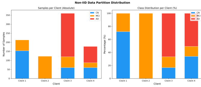
Fig. 2. Non-IID data partition across K=4 clients using Dirichlet distribution ( \alpha=0.5 ), fold 0’s training subjects only (held-out validation/test subjects for this fold are excluded from all clients). Each client receives a statistically heterogeneous subset, simulating realistic hospital demographics.
