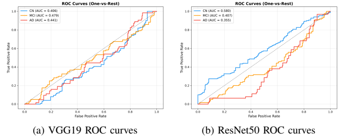
Fig. 5. Per-class ROC curves for centralised models (fold 0, seed 42). Curves cluster near the diagonal (AUROC \approx 0.45–0.46 macro-averaged), consistent with near-chance discrimination once subject-level evaluation removes slice-level leakage.
