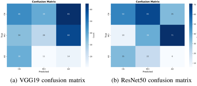
Fig. 4. Confusion matrices for centralised models on the subject-disjoint held-out test set (fold 0, seed 42). Substantial off-diagonal mass reflects the genuine difficulty of this small-cohort, subject-level classification task.
