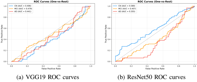
Fig. 5. Per-class ROC curves for centralised models (fold 0, seed 42). Curves cluster near the diagonal (AUROC \approx 0.45–0.46 macro-averaged), consistent with near-chance discrimination once subject-level evaluation removes slice-level leakage.
