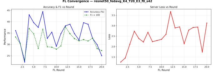
Fig. 6. Federated learning convergence for ResNet50 with K=4 clients, T=20 rounds, E=3 local epochs (fold 0, seed 42, subject-level evaluation). Validation accuracy plateaus near chance level within a handful of rounds.
