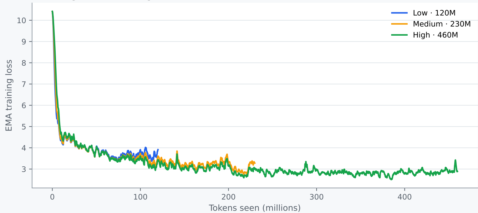
Training-loss convergence
