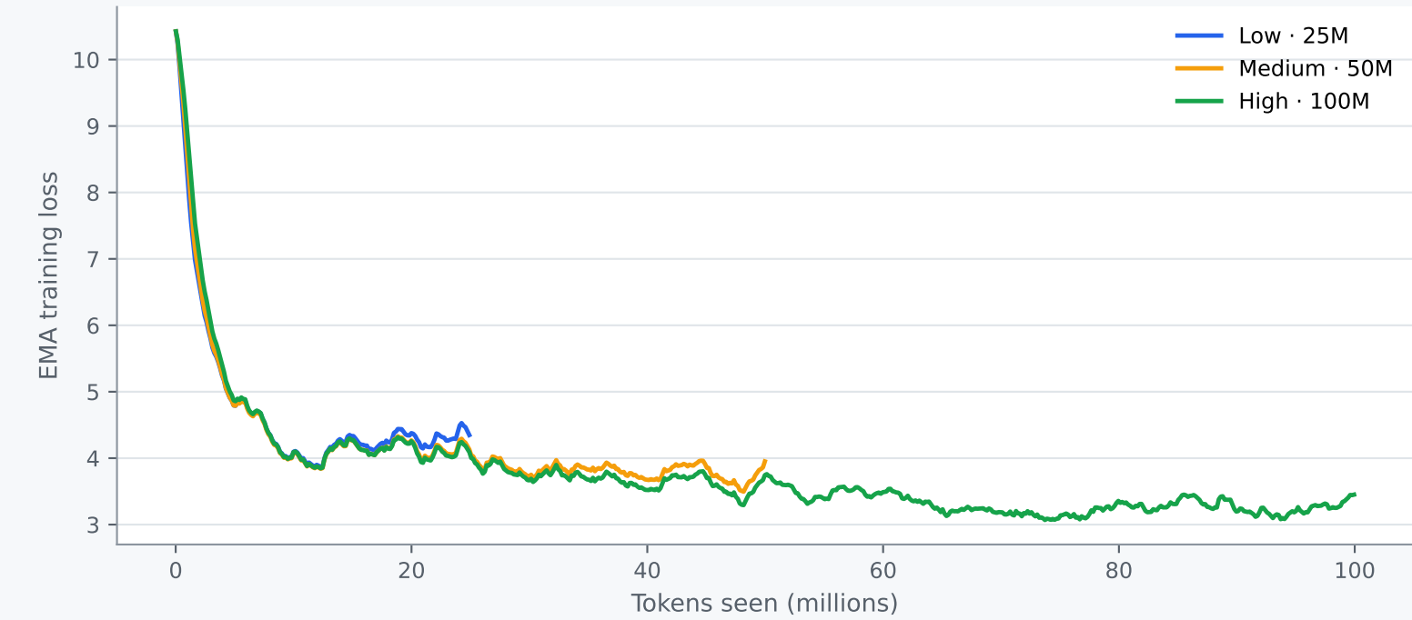
Training-loss convergence
