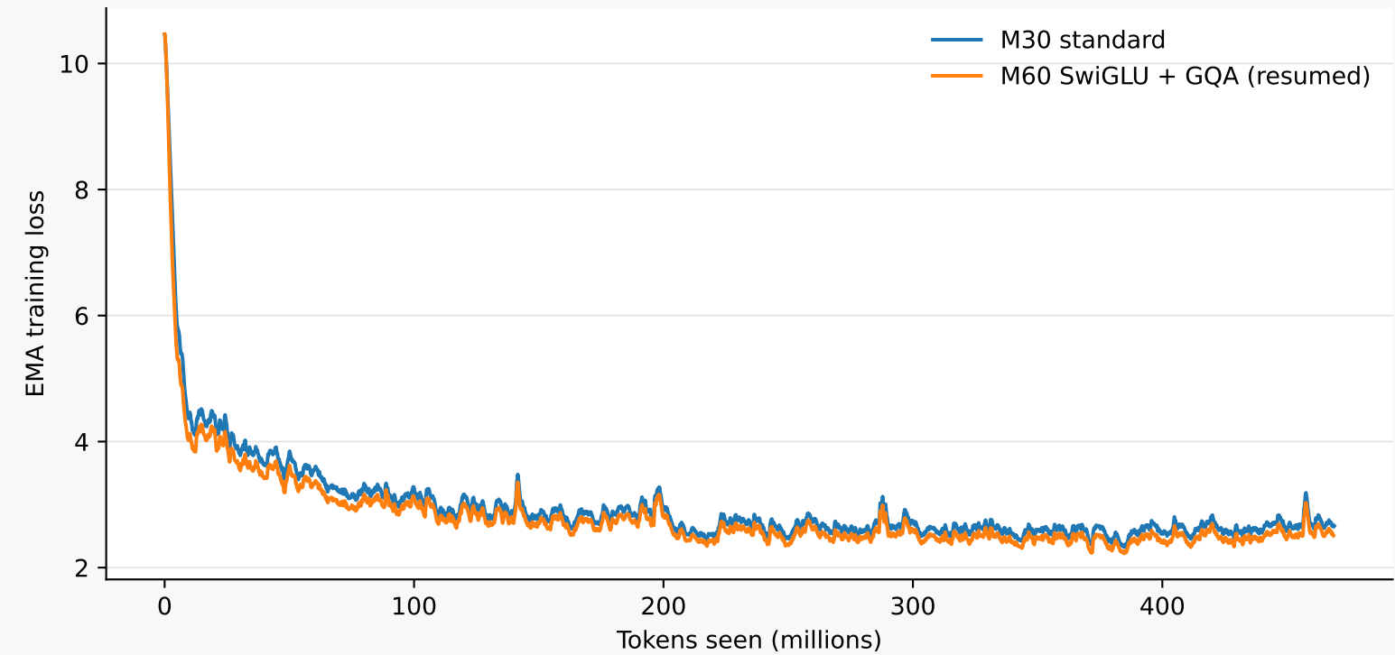
Training-loss convergence
