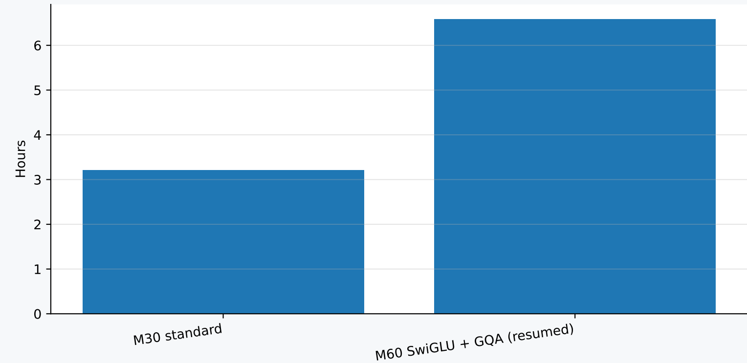
Training runtime
