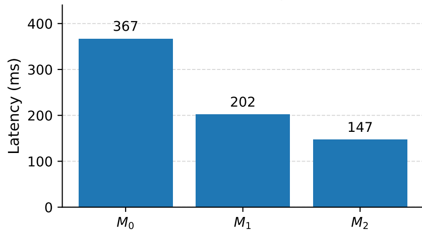
P95 Latency
