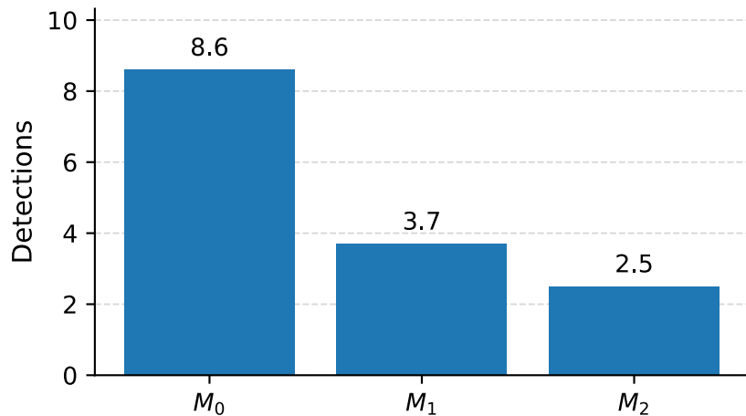
Average Detections
