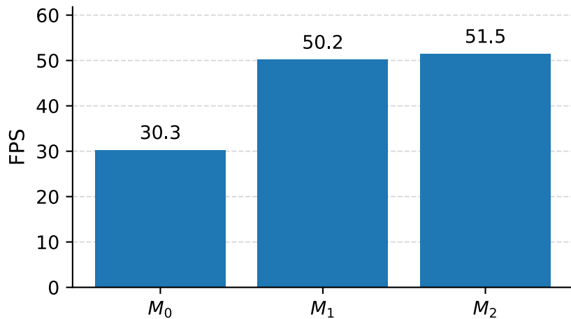
Average FPS
