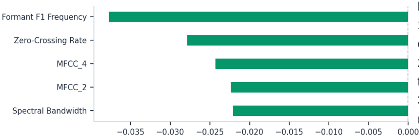
Vocal Biomarker Classifier Contributions (SHAP Values)
