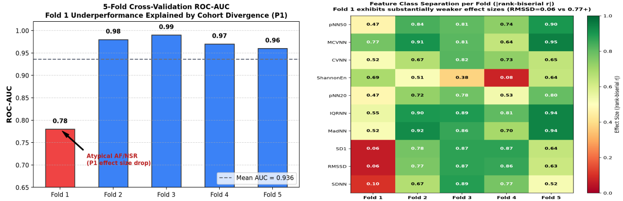
Figure 7: (Left) Cross-validation AUC per fold showing Fold 1 divergence. (Right) Feature effect size heatmap illustrating collapse of RMSSD/SD1 discriminability in Fold 1.
