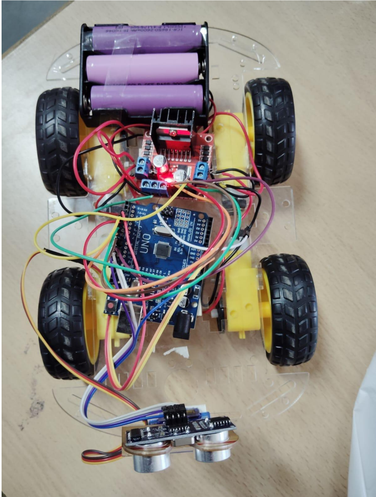
TOP VIEW OF THE CAR
