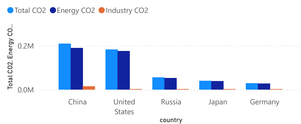
Total CO2, Energy CO2 and Industry CO2 by country
