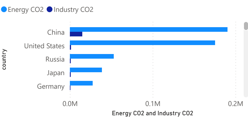
Total CO2, Energy CO2 and Industry CO2 by country
