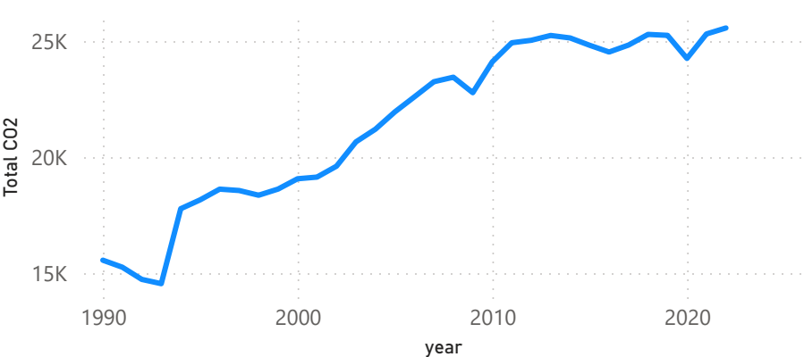
Total CO2 by year
