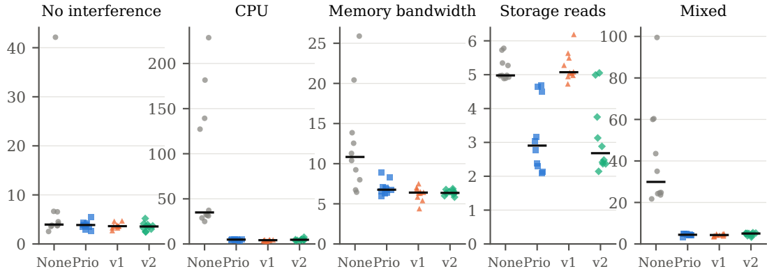
Foreground p95 latency (ms)
