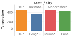
Minimum Temperature by City
