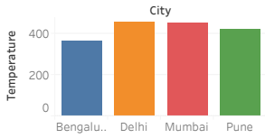
Maximum Temperature by City
