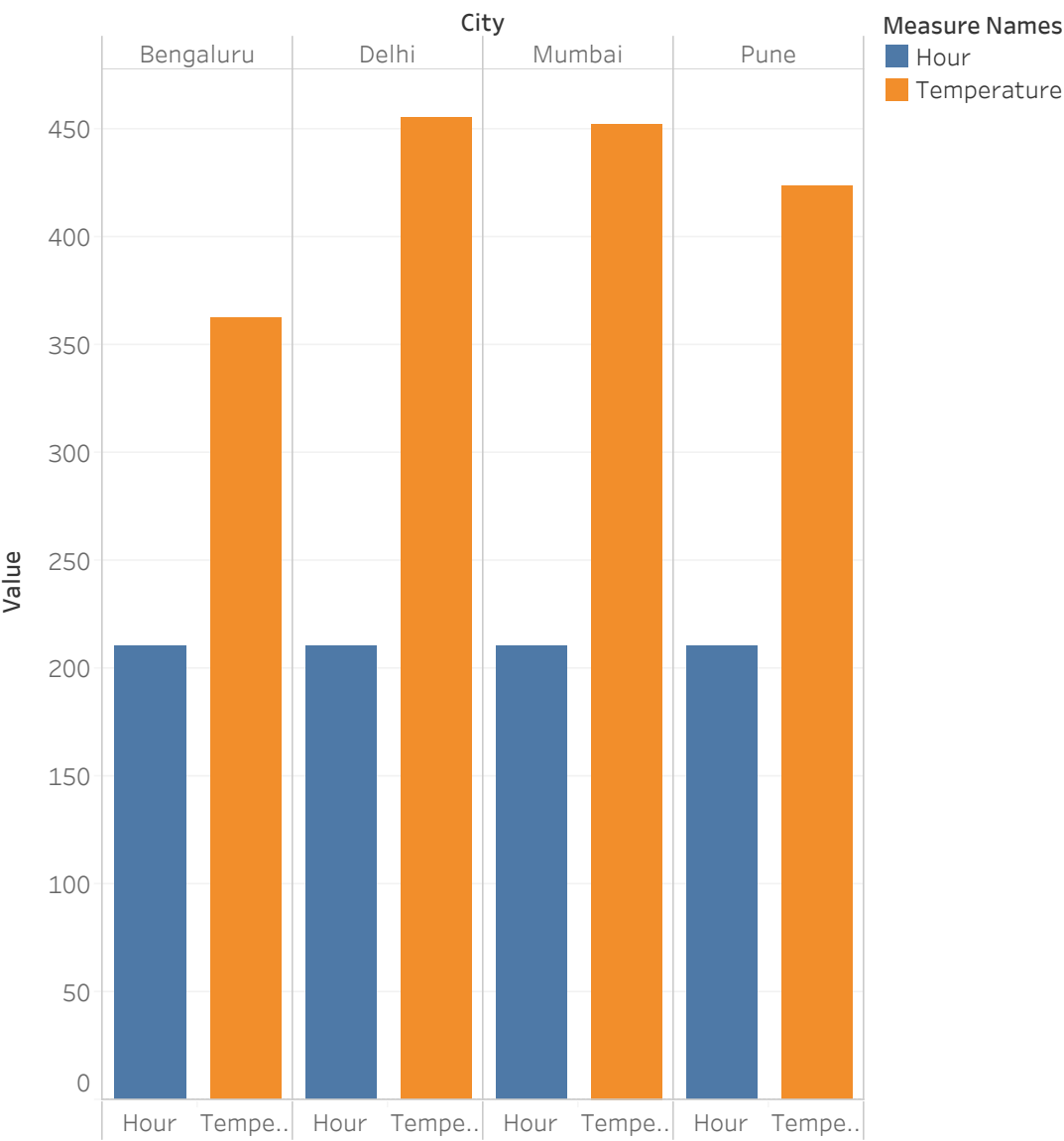
Hour and Temperature for each City. Color shows details about Hour and Temperature.
