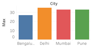
Maximum Temperature by City
