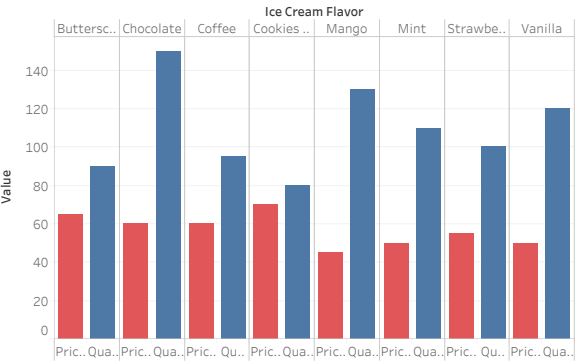
Price vs Quantity Sold
