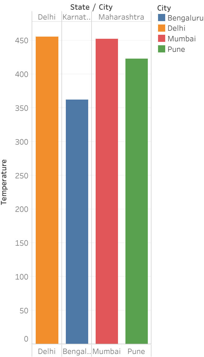
Sum of Temperature for each City broken down by State. Color shows details about City.
