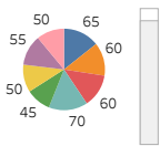
Price vs Total Sales
