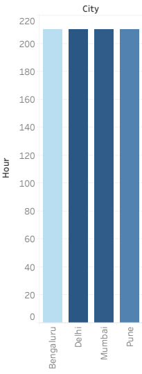
Hottest & coolest hours per city
