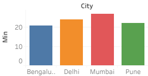
Minimum Temperature by City
