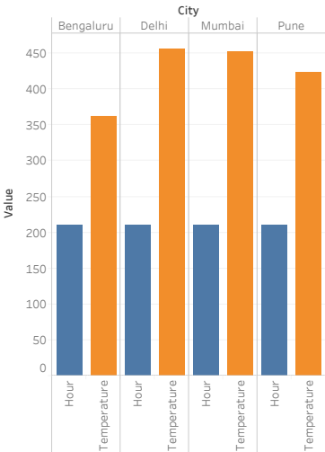
Hourly Temperature Analysis Per City
