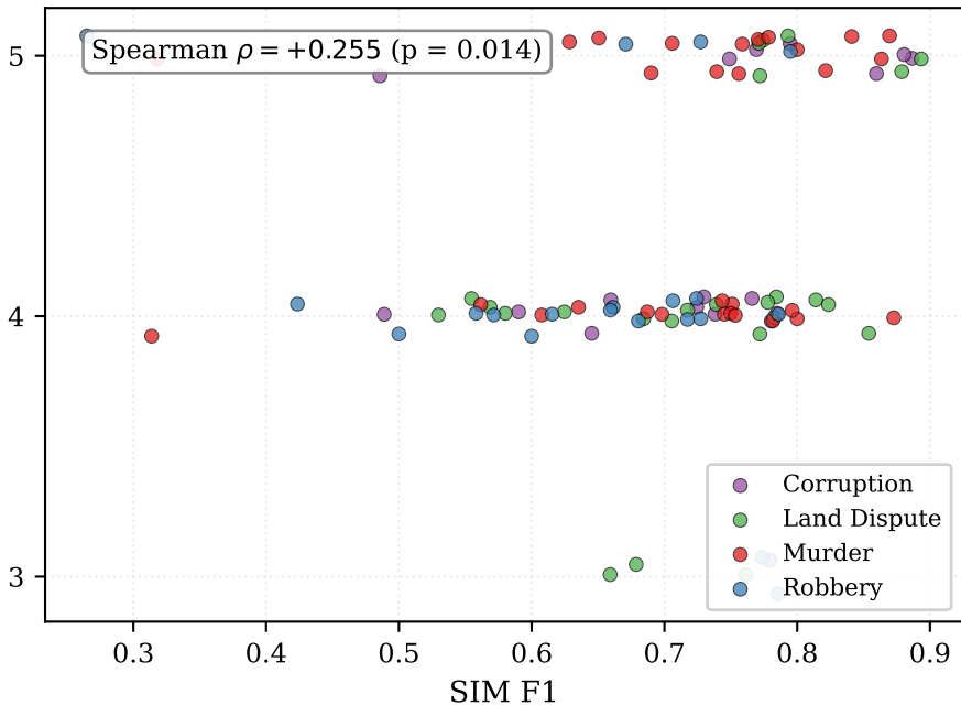
LLM-as-Judge score
