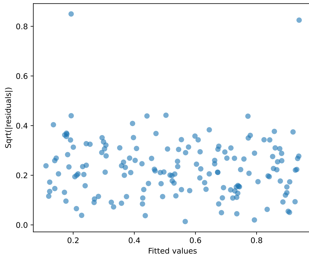
Scale-Location
