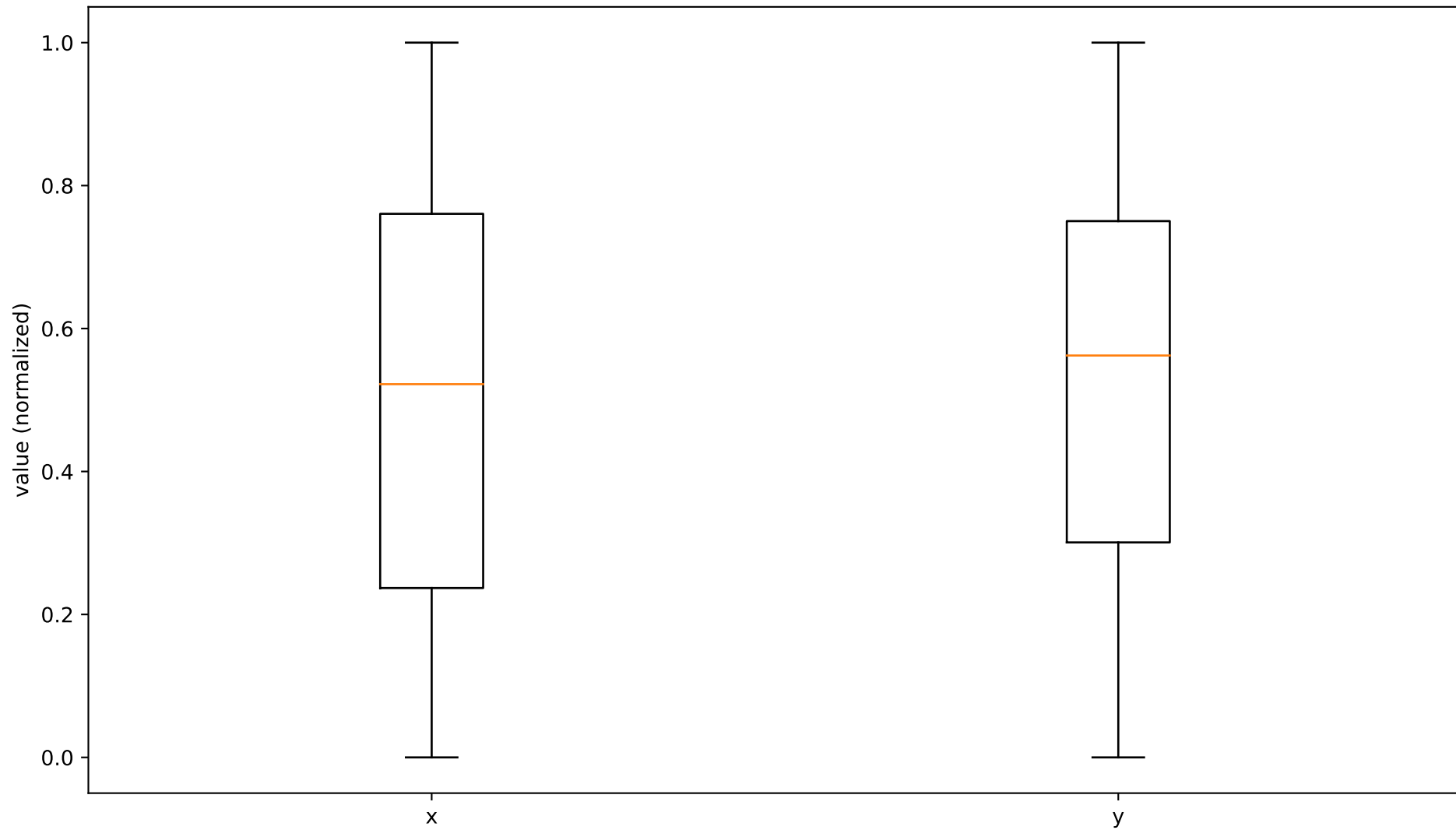
Boxplot of numeric dimensions
