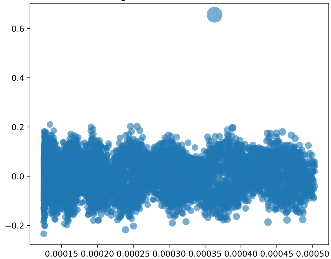
Leverage vs Residuals (size ~ Cook's)
