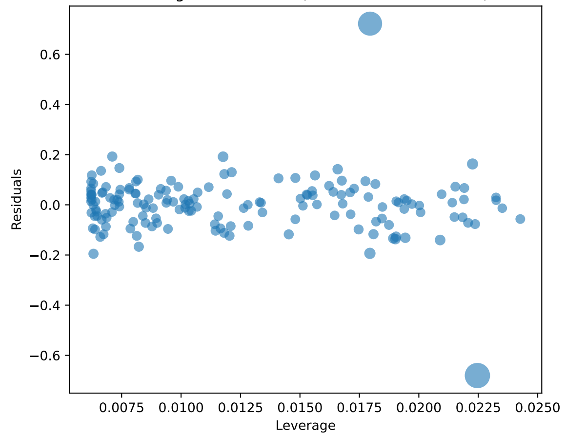
Leverage vs Residuals (size ~ Cook's distance)
