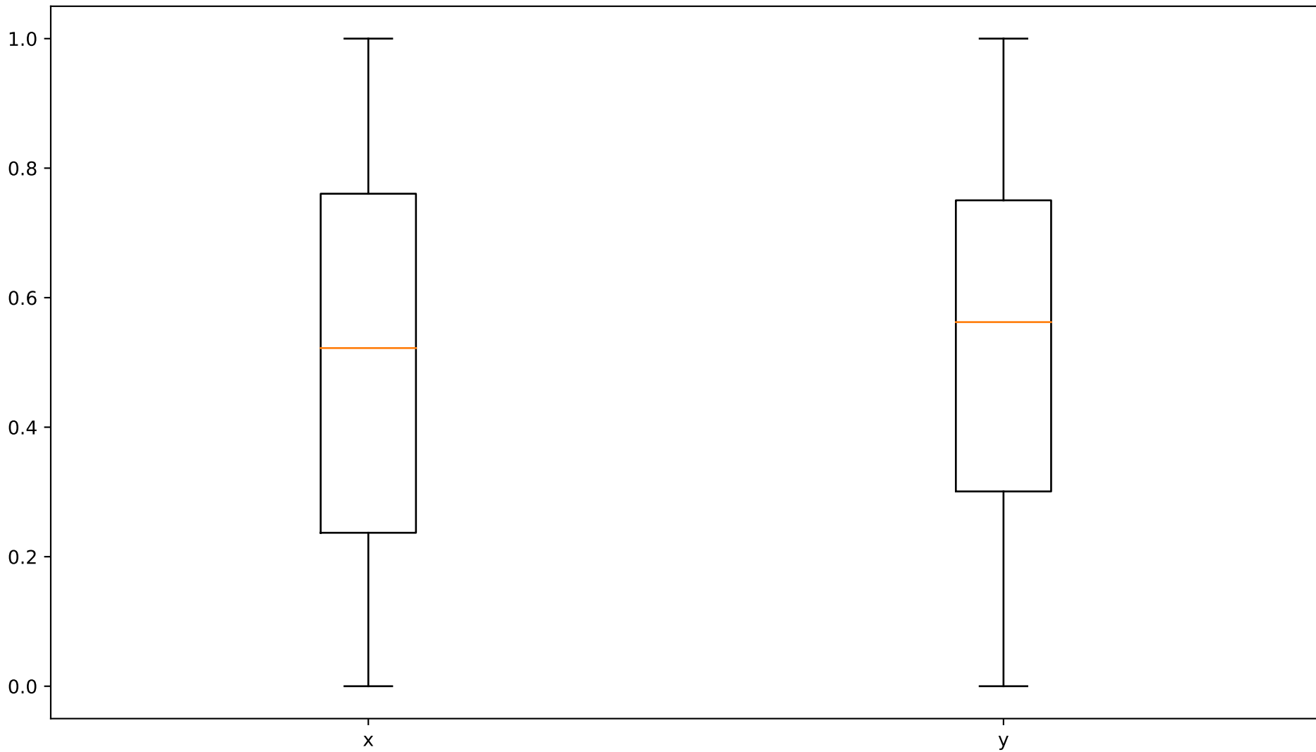
Boxplot of numeric columns
