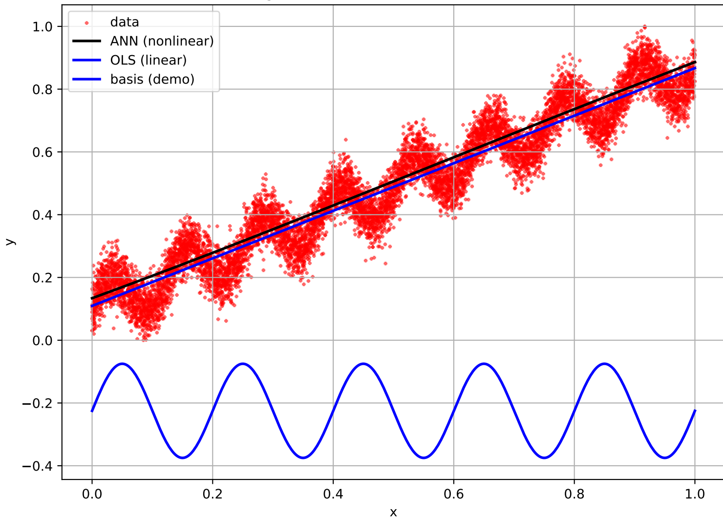
Big dataset visualization (dataset03)
