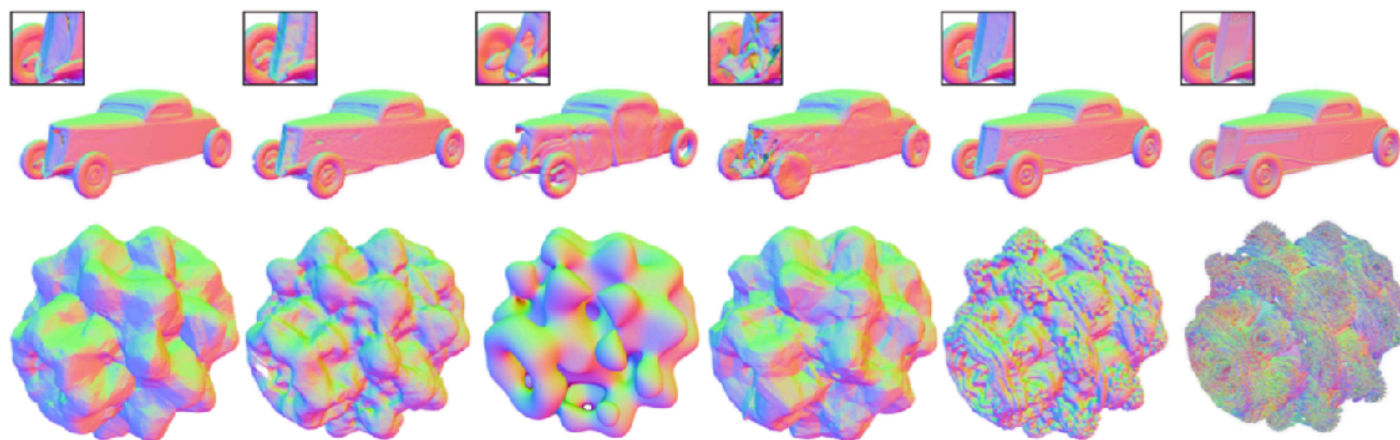
DeepSDF [39]
