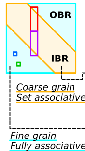
Banded Matrix
