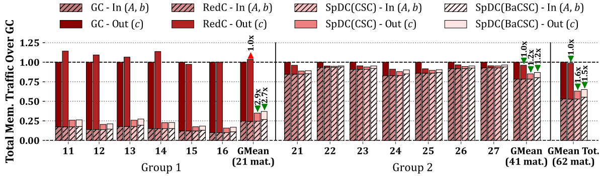
Figure 5.8: Total Memory Traffic on Input Matrix A , Input Vector b and Output Vector c , Normalized over GC, from RTL Simulations
