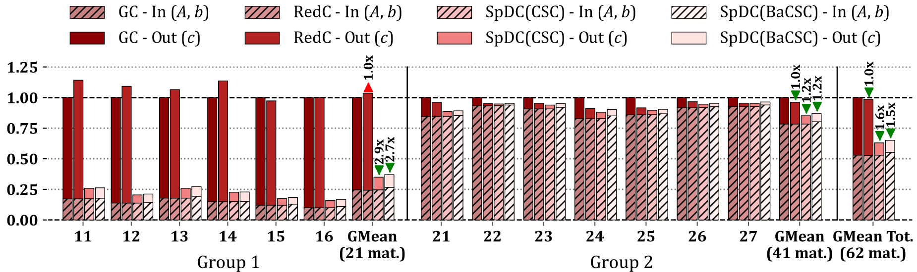
Total Mem. Traffic Versus GC
