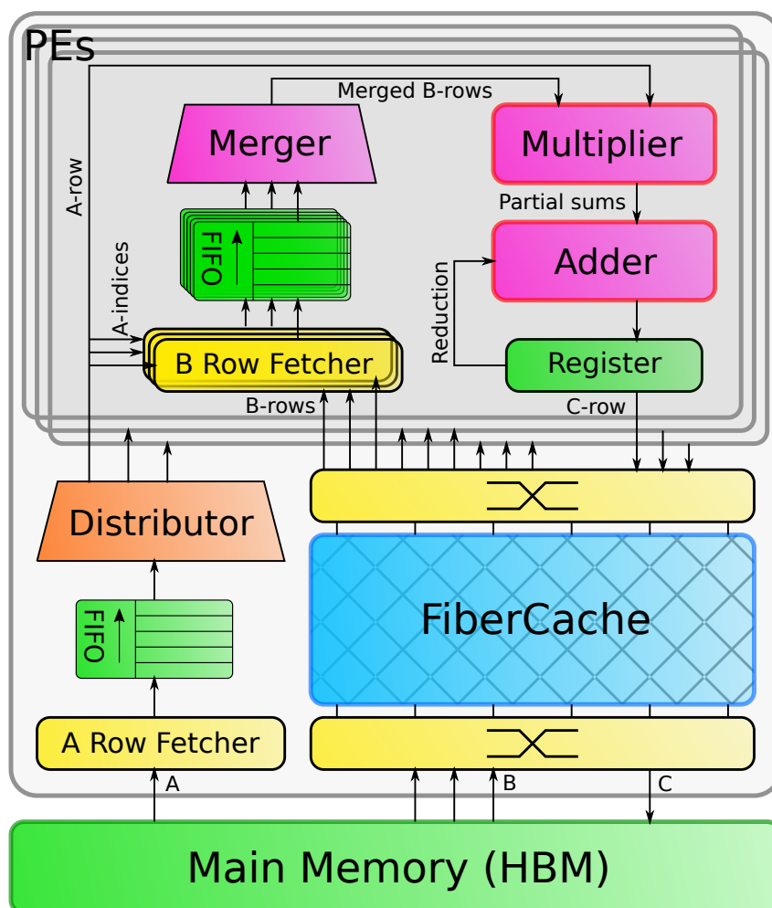
Figure 2.4 – Architecture of Gamma
