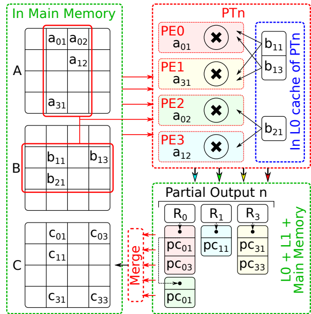
Figure 2.2 – OuterSPACE Data Flow
