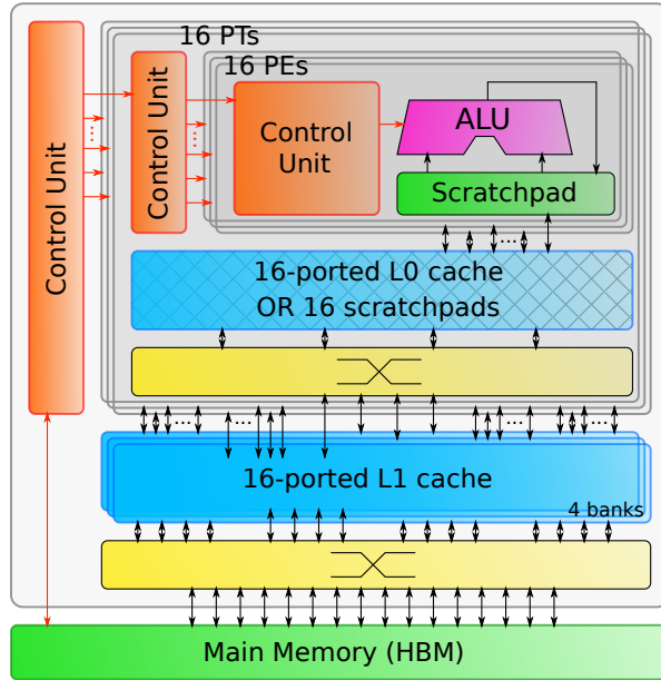
Figure 2.1 – Architecture of OuterSPACE
