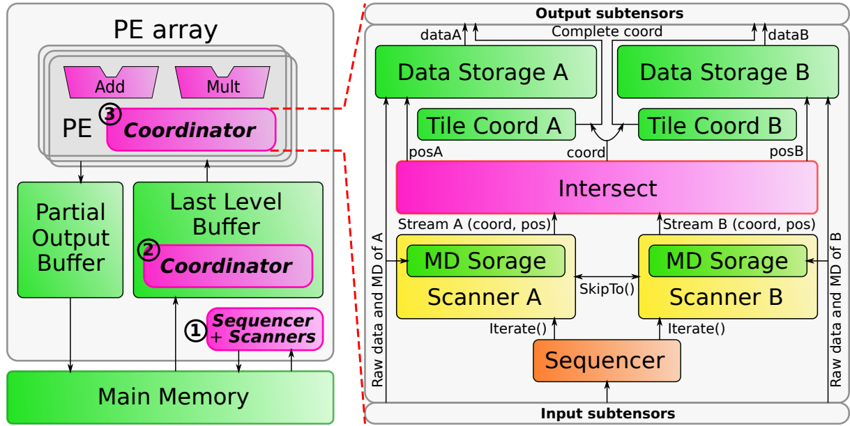
Figure 2.3 – Architecture of ExTensor
