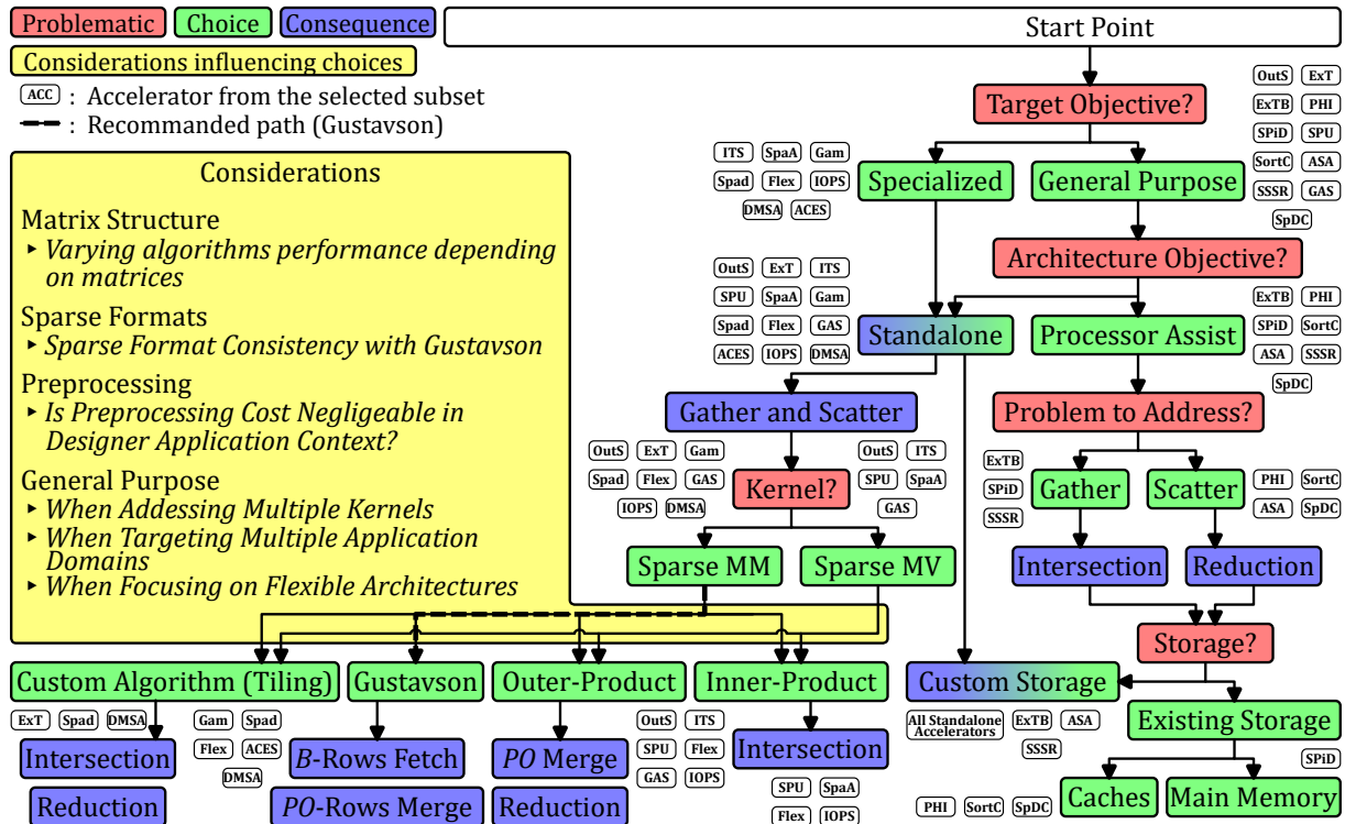
Figure 2.5 – Flow Diagram for Architecture Selection
