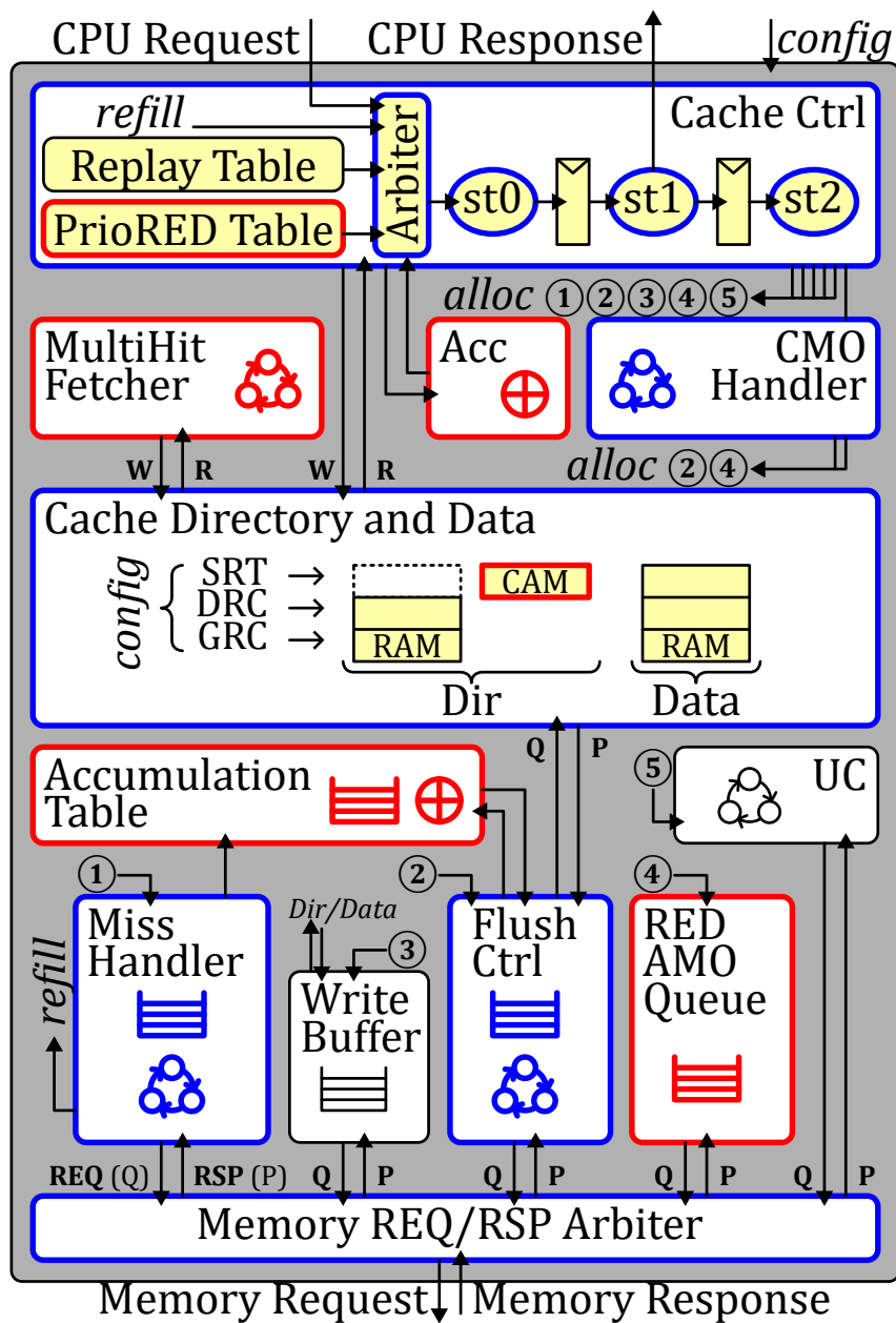
Figure 5.1: SpDCache Microarchitecture, based on HPDcache RMWQ
