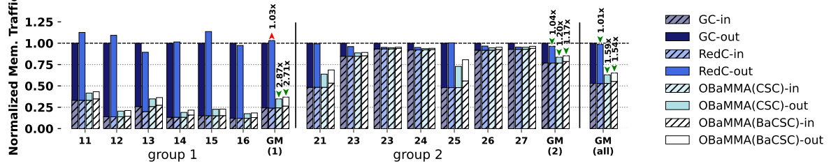
Figure 5.8: Normalized Memory Traffic on Input Matrix, Input Vector and Output Vector
