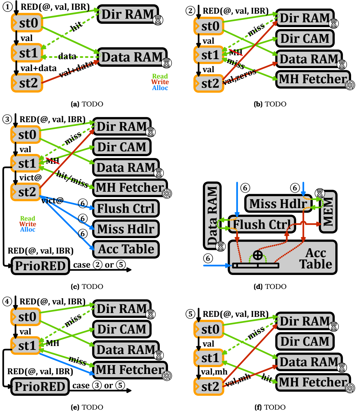
Figure 5.3: Pipeline Operation IBR
