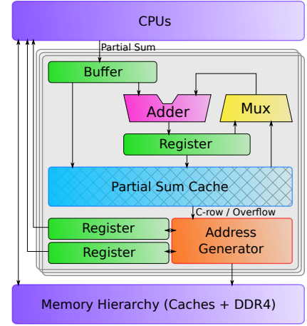
Figure 2.11: Architecture of ASA
