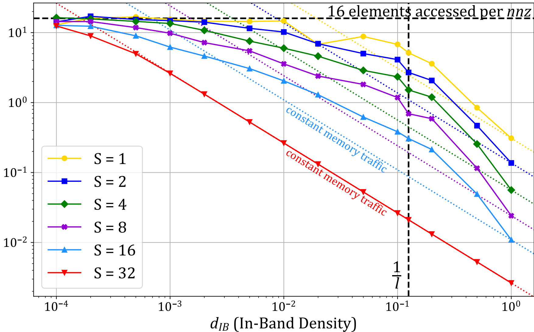
Normalized Memory Traffic
