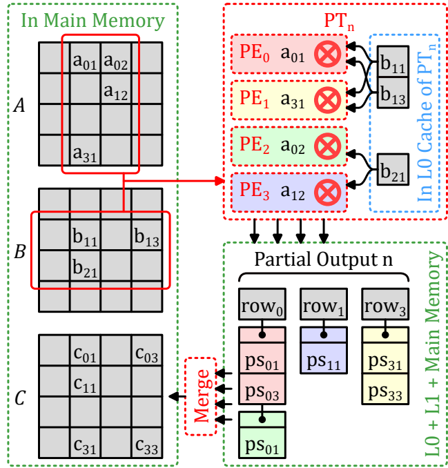
Figure 2.2 – OuterSPACE Dataflow
